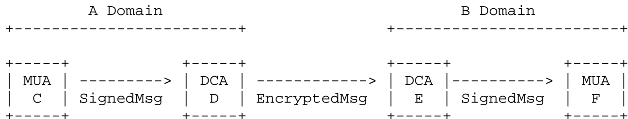
Figure 1: Architecture of Secure Headers
