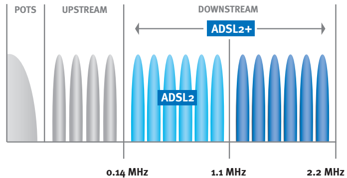
Figure 7: ADSL2+ doubles the bandwidth used to carry data.
