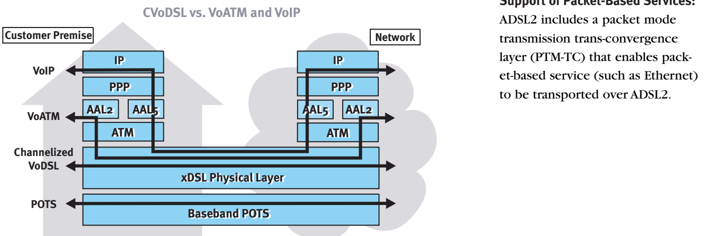
Figure 6: CVoDSL does not packetize voice data, as VoIP and VoATM do.
