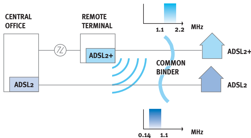
Figure 9. ADSL2+ can be used to reduce crosstalk.
