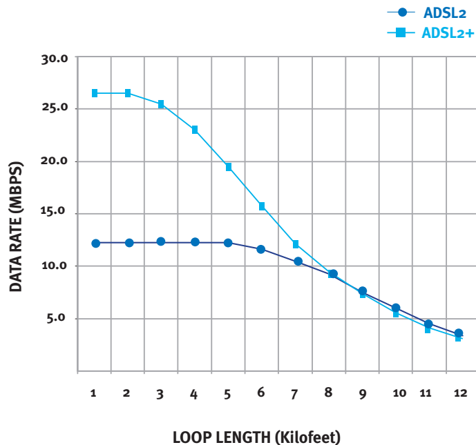
Figure 8: ADSL2+ doubles the maximum data rate.
