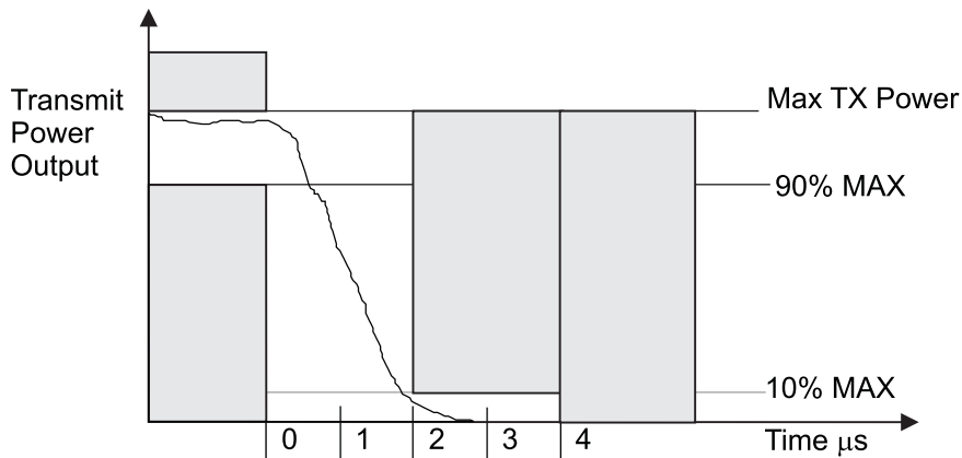
Figure 98—Transmit power-down ramp
