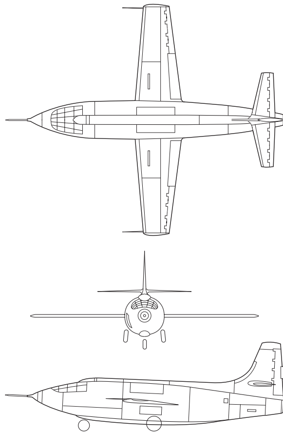
NACA X-1 Research Aircraft 1946
